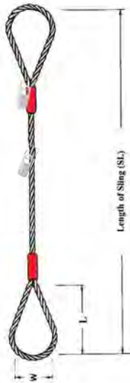
Single Leg Redi-Grip® Sling
